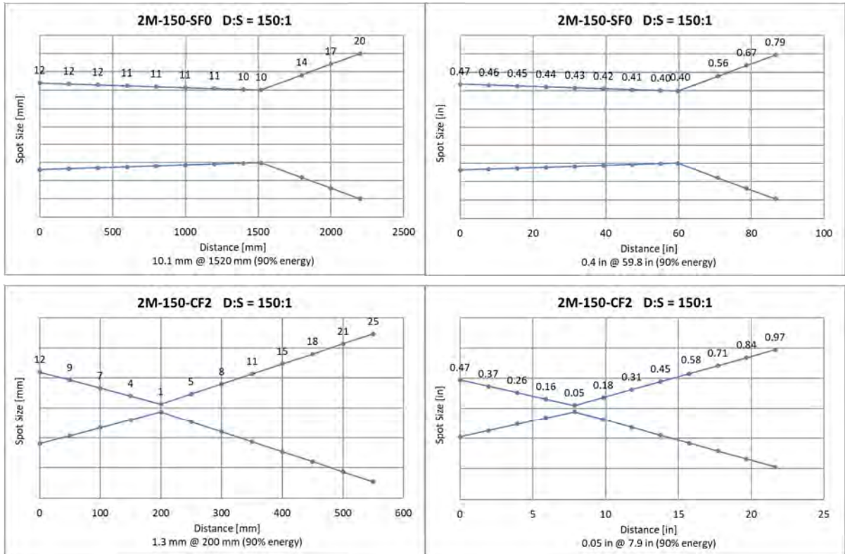
Figure 15-20: Optical Diagrams 2M-150 Models
