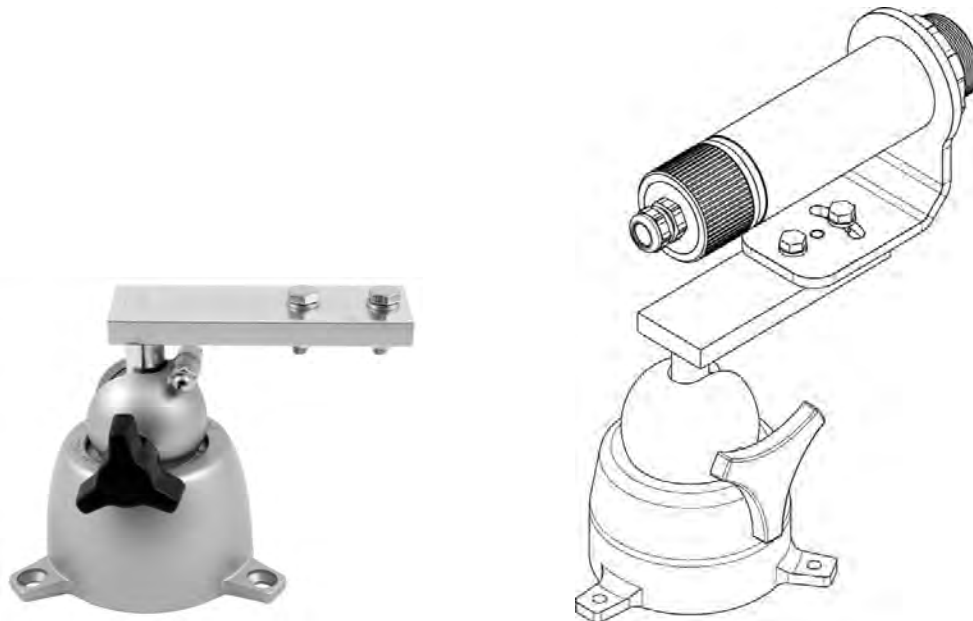
Figure 13-15: Swivel Bracket
