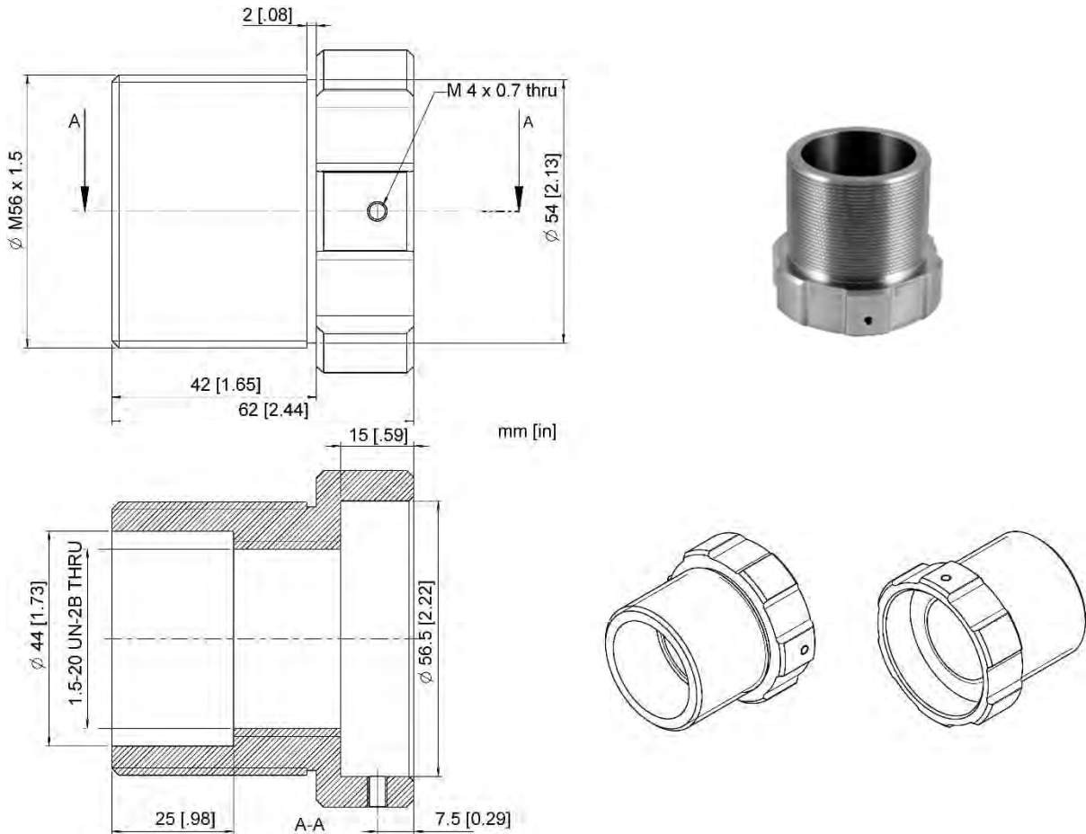
Figure 13-24: Thread Adapter
