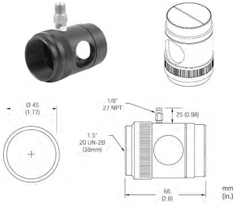
Figure 13-21: Right Angle Mirror
