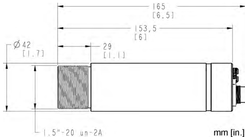
Figure 2-3: Dimensions for the 12-Wire Model
