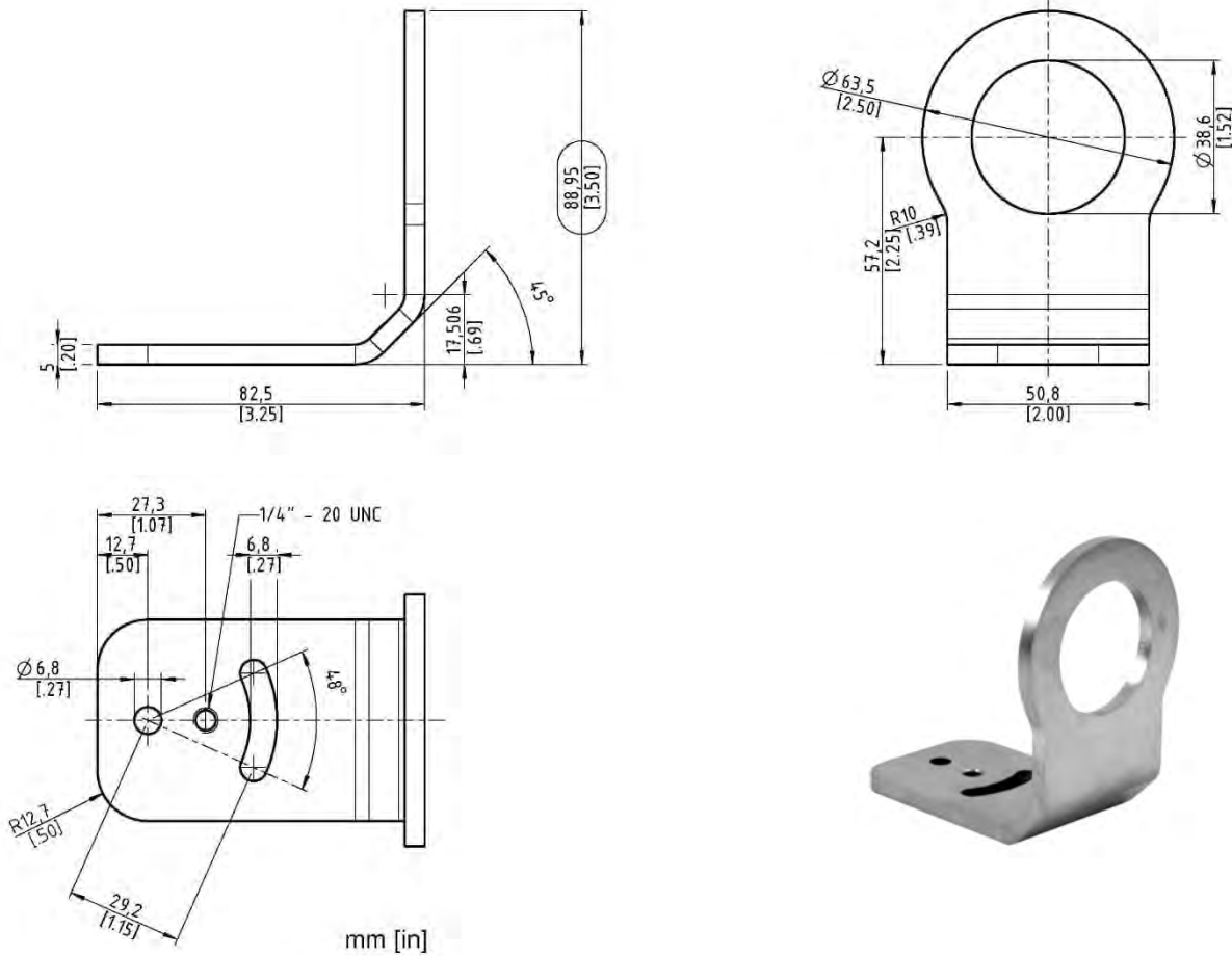
Figure 13-13: Fixed Bracket
