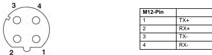
Figure 5-9: M12 Connector Socket and Pin Assignment
