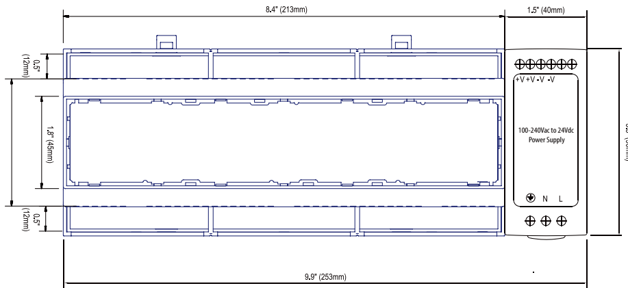
Figure 1 - Top View
