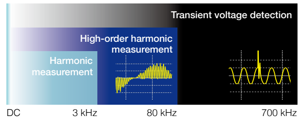
The PQ3198's wideband capability extends from DC voltages to 700 kHz.
