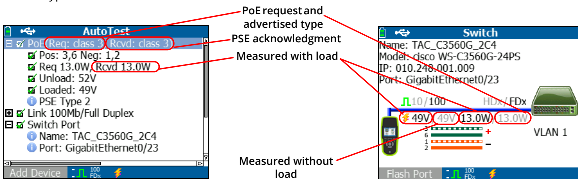
Figure 23. AutoTest results - PoE with TruePower
