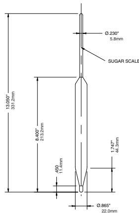
Beer Hydrometer
