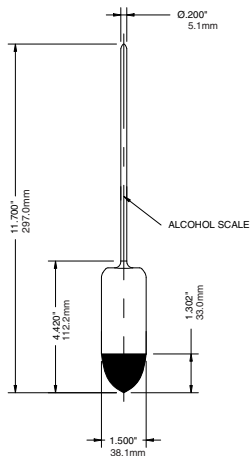
Alcohol Hydrometer
