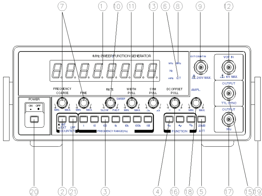
FIG 1-2. FRONT PANEL OPERATOR'S CONTROLS(FG-7005C,)
