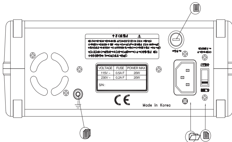
FIG 2-2. REAR PANEL(FG-7005C)
