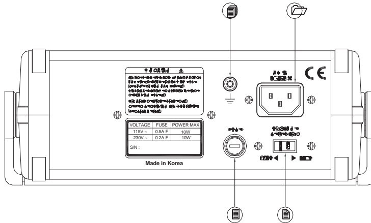
FIG 2-1. REAR PANEL(FG-7002C)
