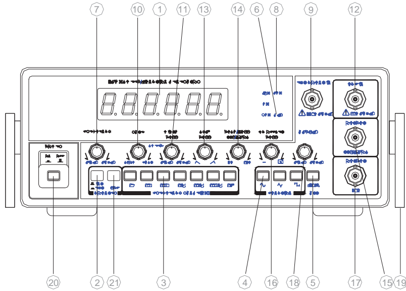
FIG 1-1. FRONT PANEL OPERATOR'S CONTROLS(FG-7002C)
