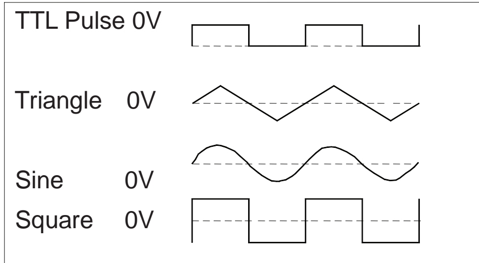
FIG. 3 OUTPUT WAVEFORMS AND PHASE RELATIONSHIPS
