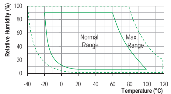
Operating conditions
