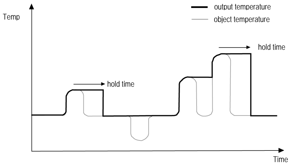
Figure 22: Peak Hold
