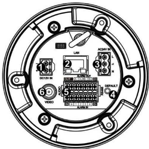
CP-6408-21-I Connectors
