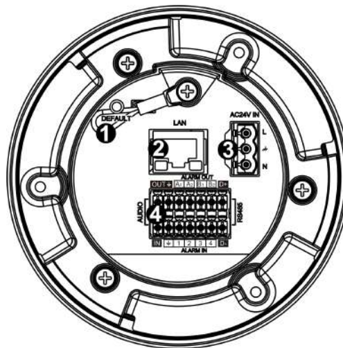
CP-6408-31-I Connectors
