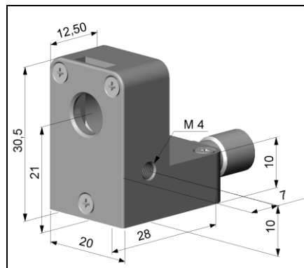
Laminar air purge collar – the sideward air outlet prevents a cooling down of the object in short distances; hose connection: 3x5 mm [ACCTAPL]
