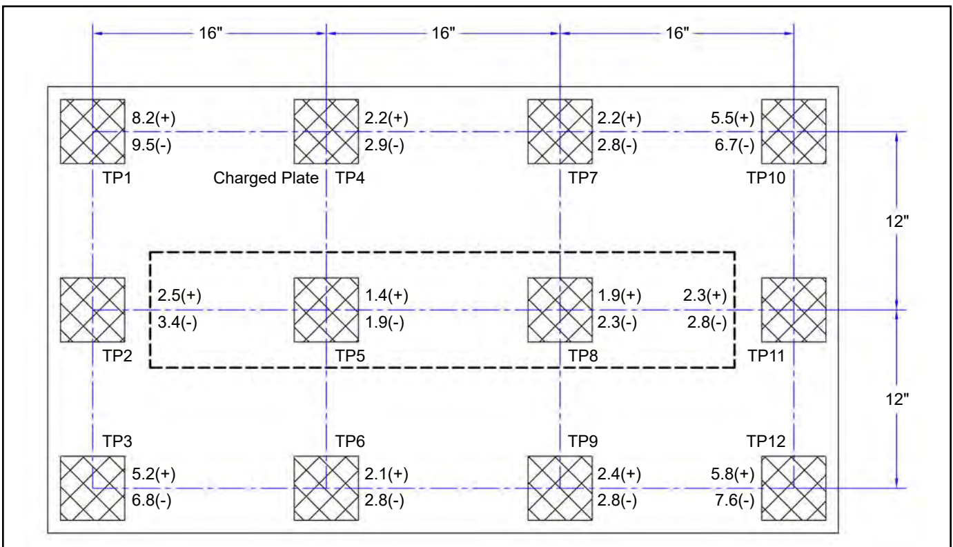
Figure 13. 770113 Neutralization (Discharge) Times at 120VAC, 60Hz input
