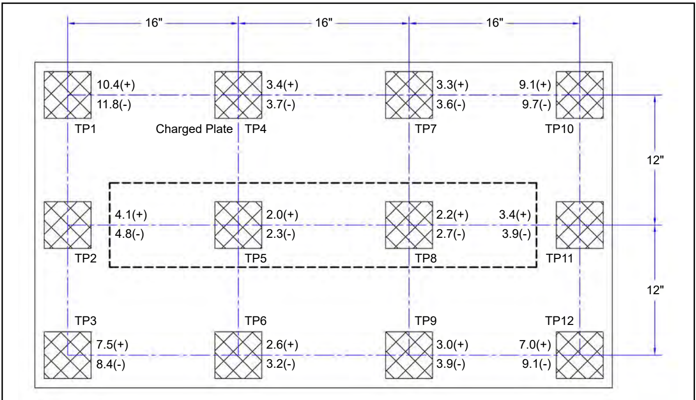
Figure 12. 770113 Neutralization (Discharge) Times at 100VAC, 50Hz input
