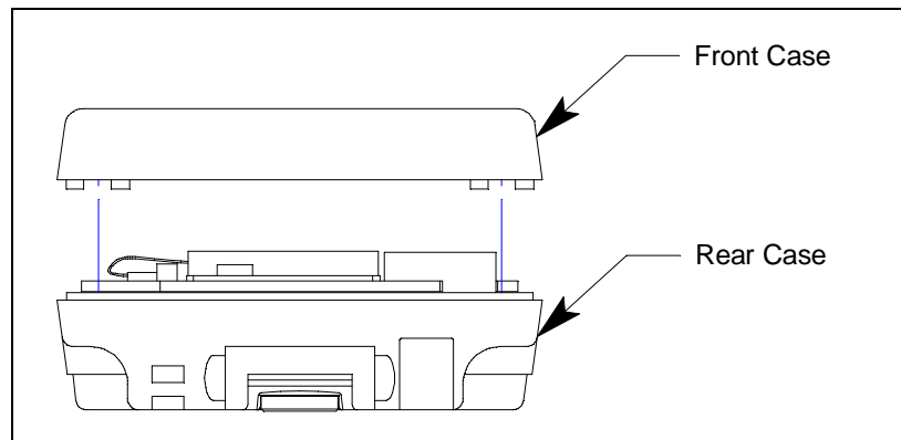
Figure 15: Case Separation
