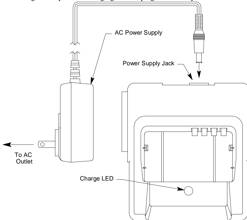
Figure 21: Connecting the Charging Station's AC Adapter
