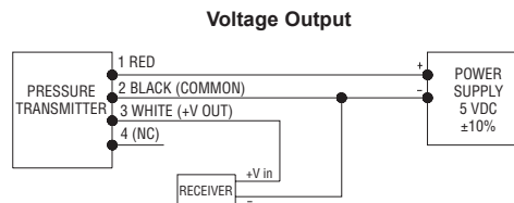
Fig. J: Voltage output connection
