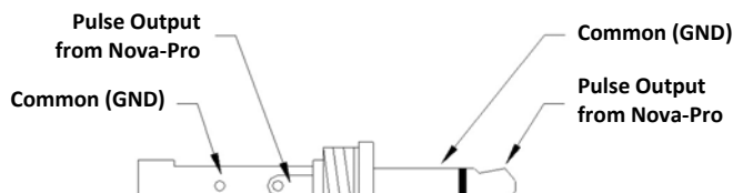
Figure 4 Output Connector Detail (Mono plug)
