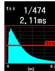
Flash Duration Analysis Cordless Mode Flash Waveform Graph Screen
