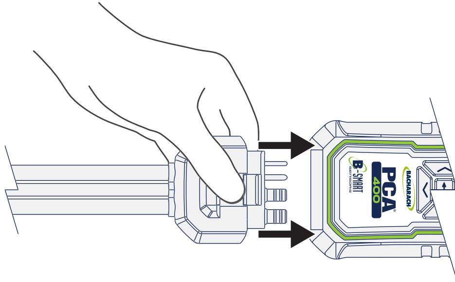
Fig. 3-3: Insert Gray Quick-Connector into Analyzer
