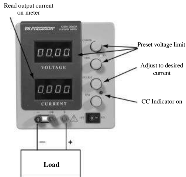
Figure 6. Typical Constant Current Operation.
