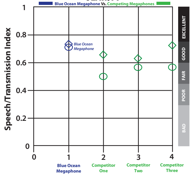
Comparison of Speech Transmission Index measured at 93.5 feet (diamond) and 186 feet (circle)
